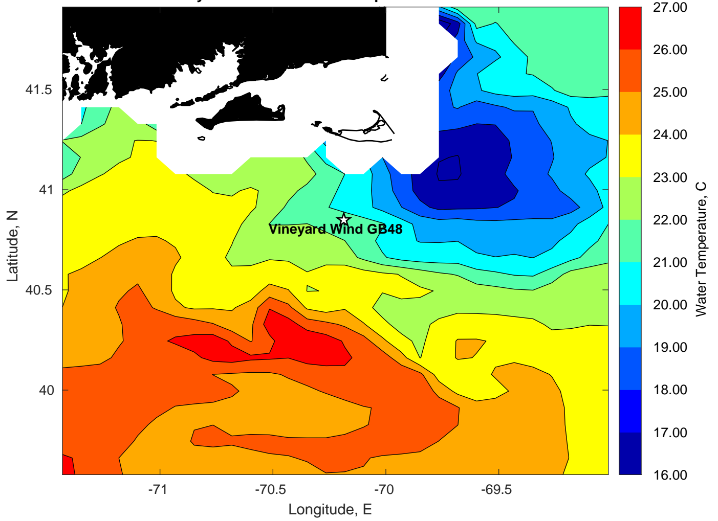
SST for Vineyard Wind GB48 at 07-Sep-2022 00:00:00
